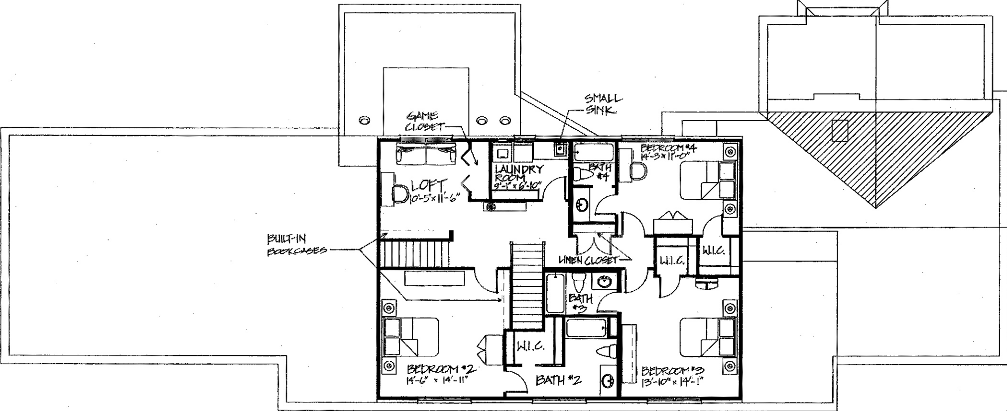
62 Portland Drive Second Floor 1,258 square feet
